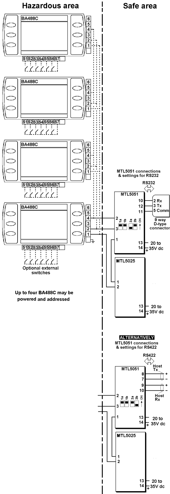
Fig 5 Three wire system for RS232 or RS422
